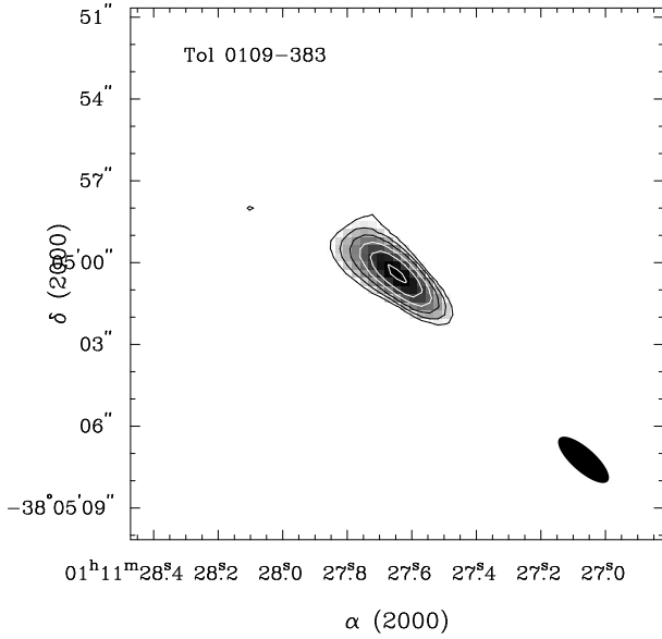
Fig. 5. TOL 0109-383. Contours: -1.0, -0.6, 0.6, 1, 1.7, 3, 5, 9 mJy beam -1
